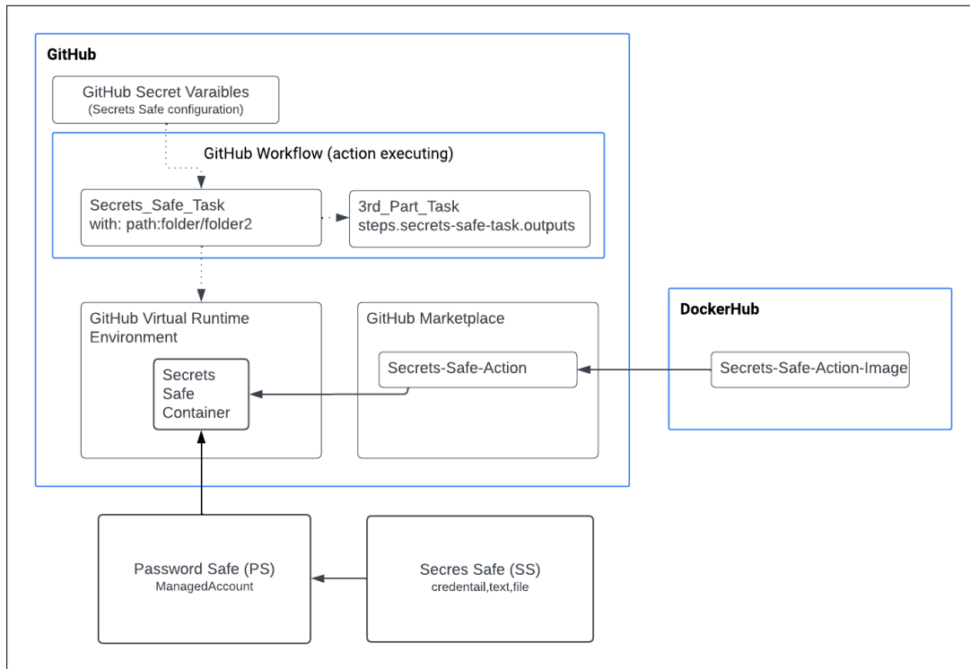
Figure 4 – GitHub Integration Workflow.
